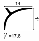
C991 Purotouch® 200 x 11 x 14 cm Designed by Ulf Moritz
